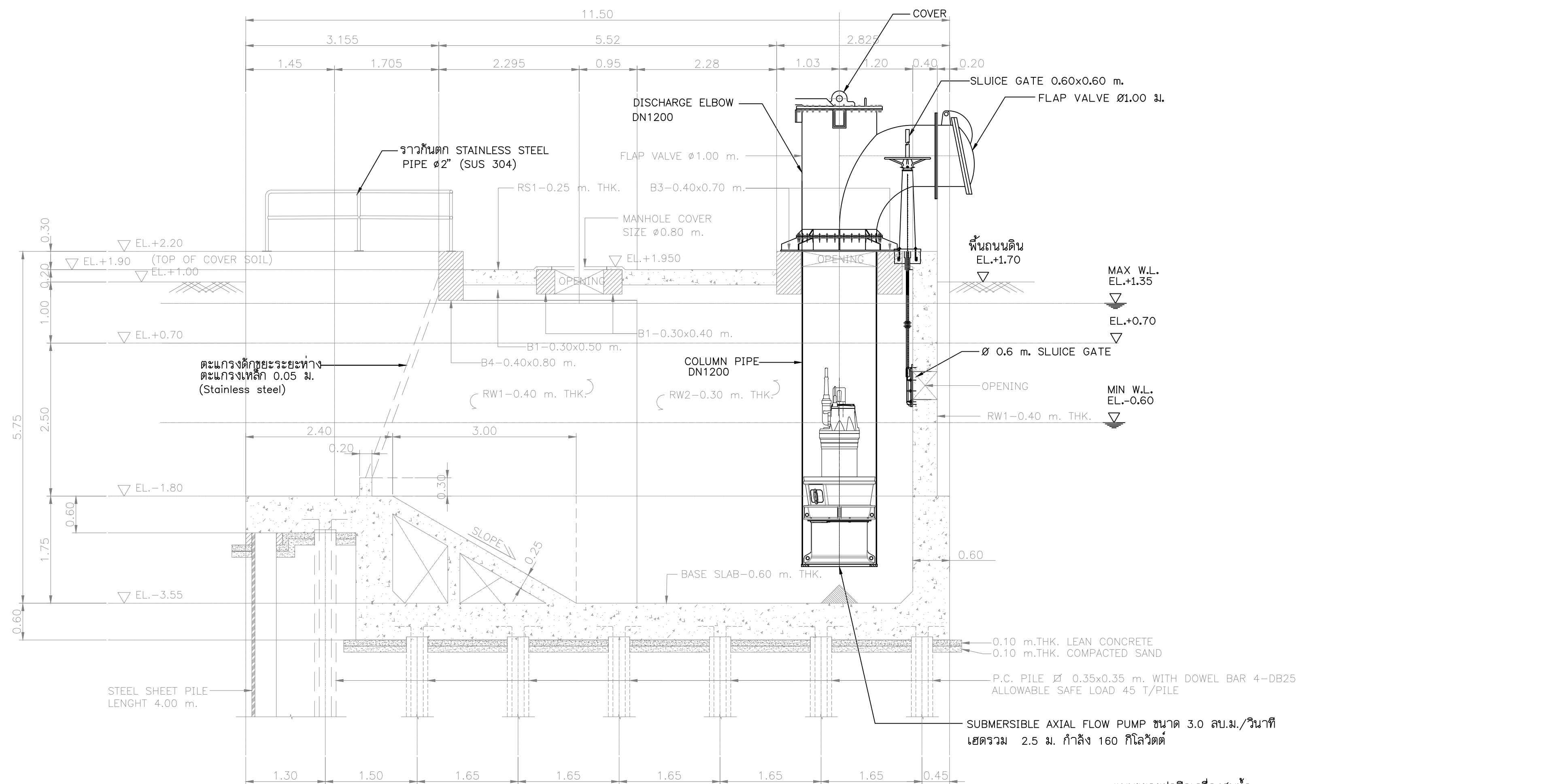
SECTION A SCALE 1:50
