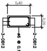
BEAM RB1B SCALE 1:20
