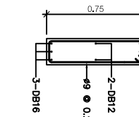
BEAM B5 SCALE 1:20
