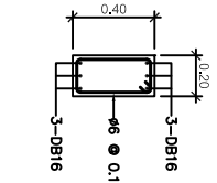
BEAM B3 SCALE 1:20
