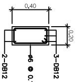
BEAM B2 SCALE 1:20
