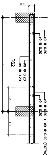
SLAB RS2 SCALE 1:20
