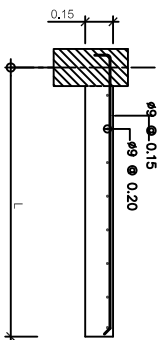
SLAB S1A SCALE 1:20
