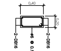
BEAM B4 SCALE 1:20
