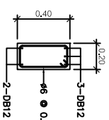
BEAM RB1A SCALE 1:20
