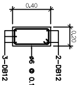
BEAM B1A SCALE 1:20
