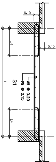
SLAB S1 SCALE 1:20
