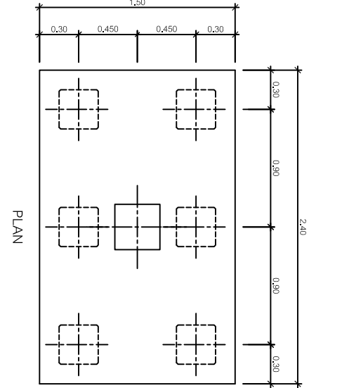
FOOTING DETAIL "F2"
