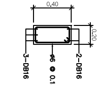
BEAM B2 SCALE 1:20
