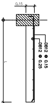
SLAB S1B SCALE 1:20
